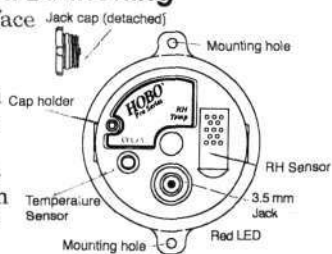
Diagram A - HOBO Pro Series Front
